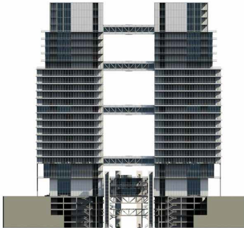
SOUTH ELEVATION
